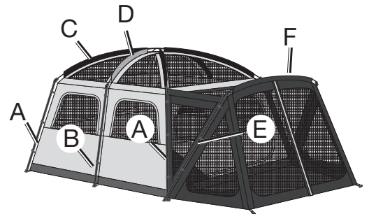
Tent without rainfly
