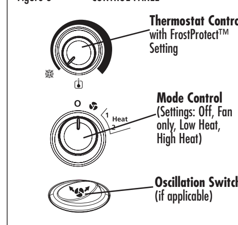
Figure 6 CONTROL PANEL
